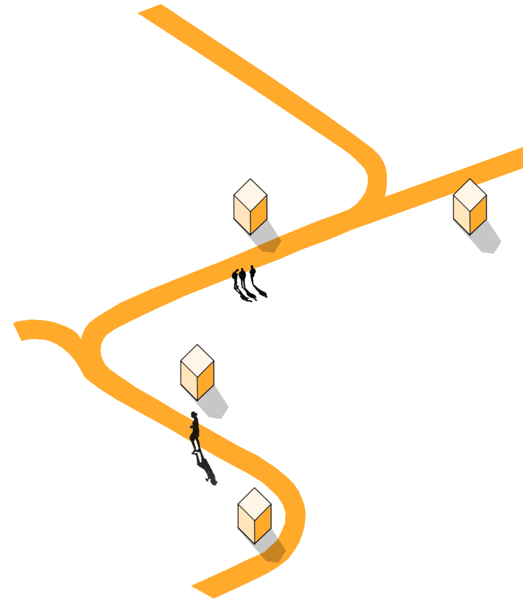
Phase 2
