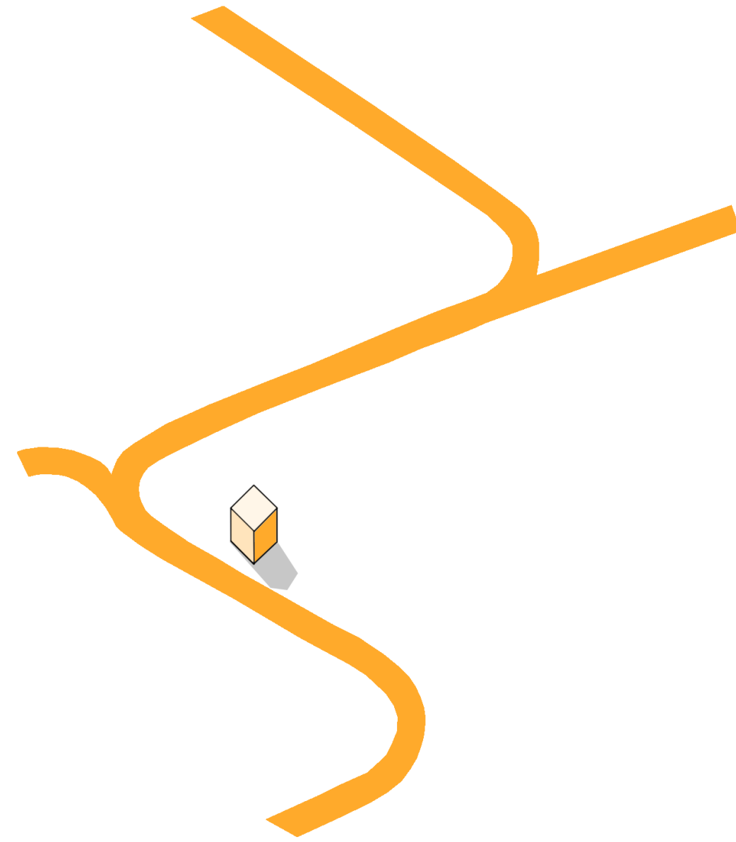
Phase 1
