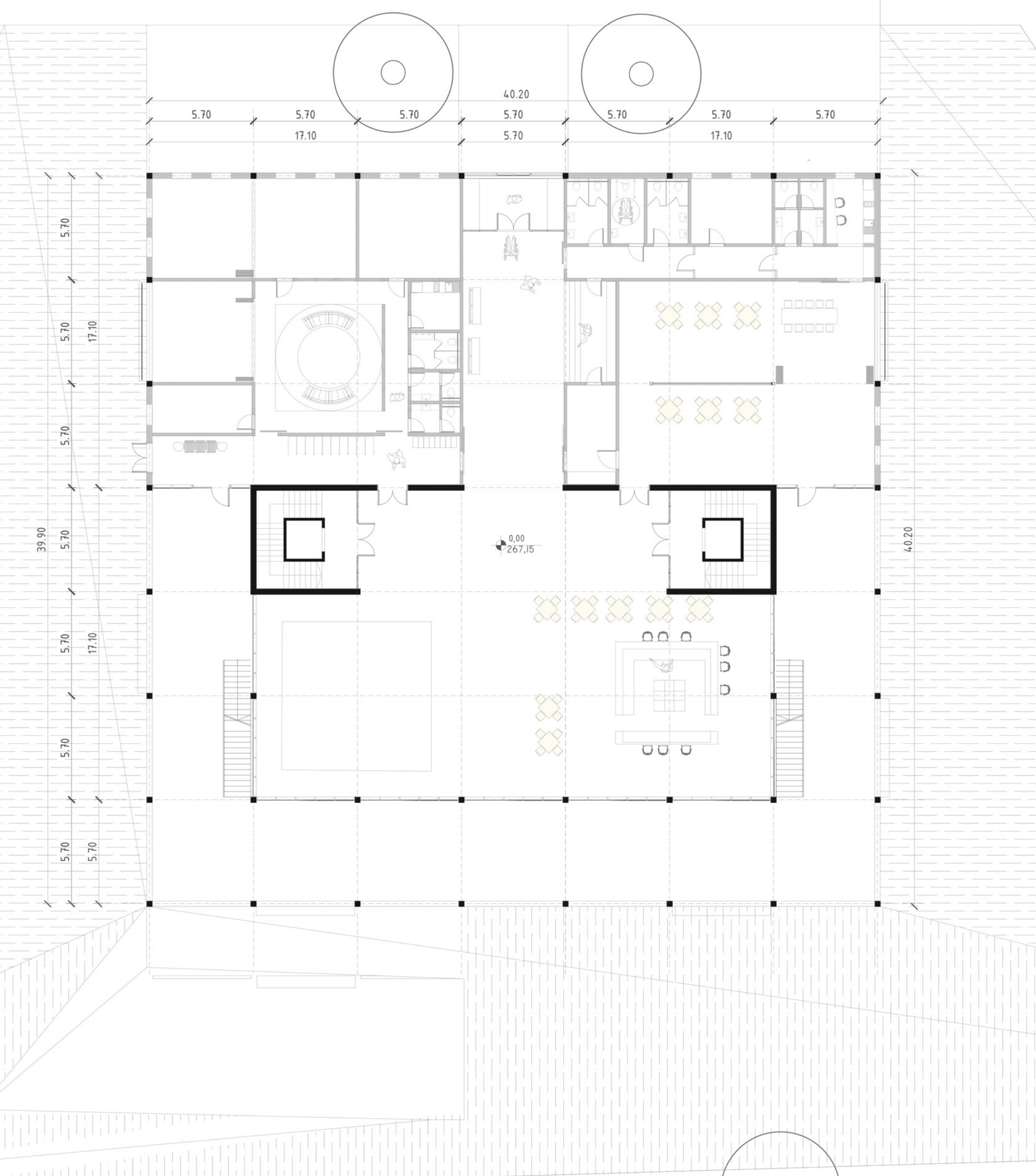
Ground Floor Plan 1:200
