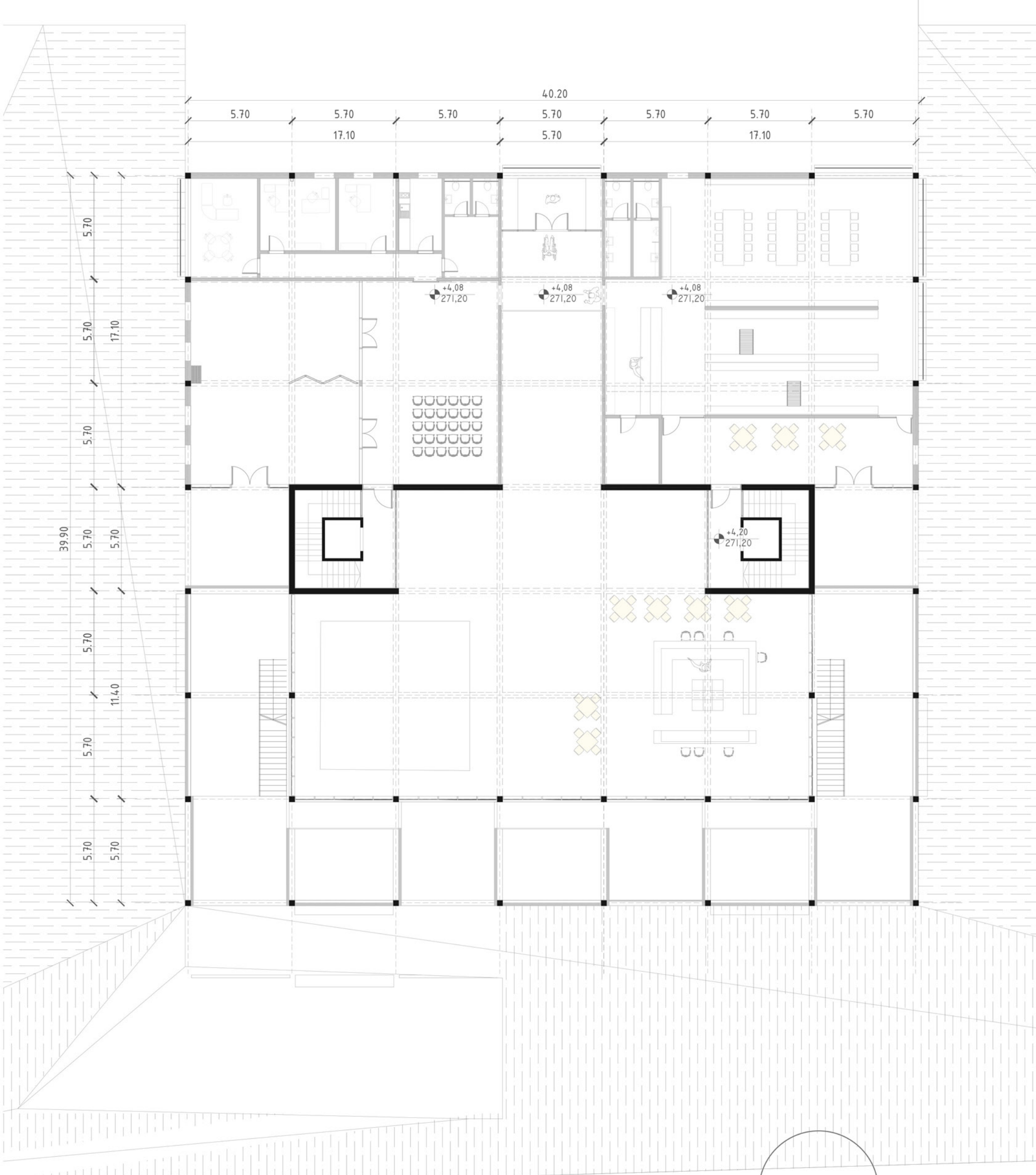
Floor Plan 1:200
