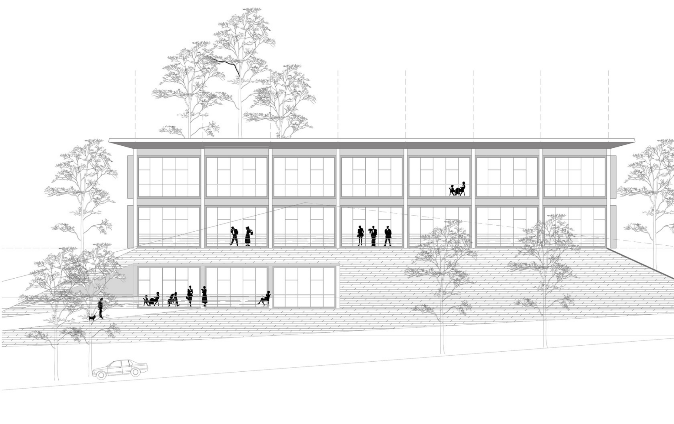
Southern Facade Elevation 1:200
