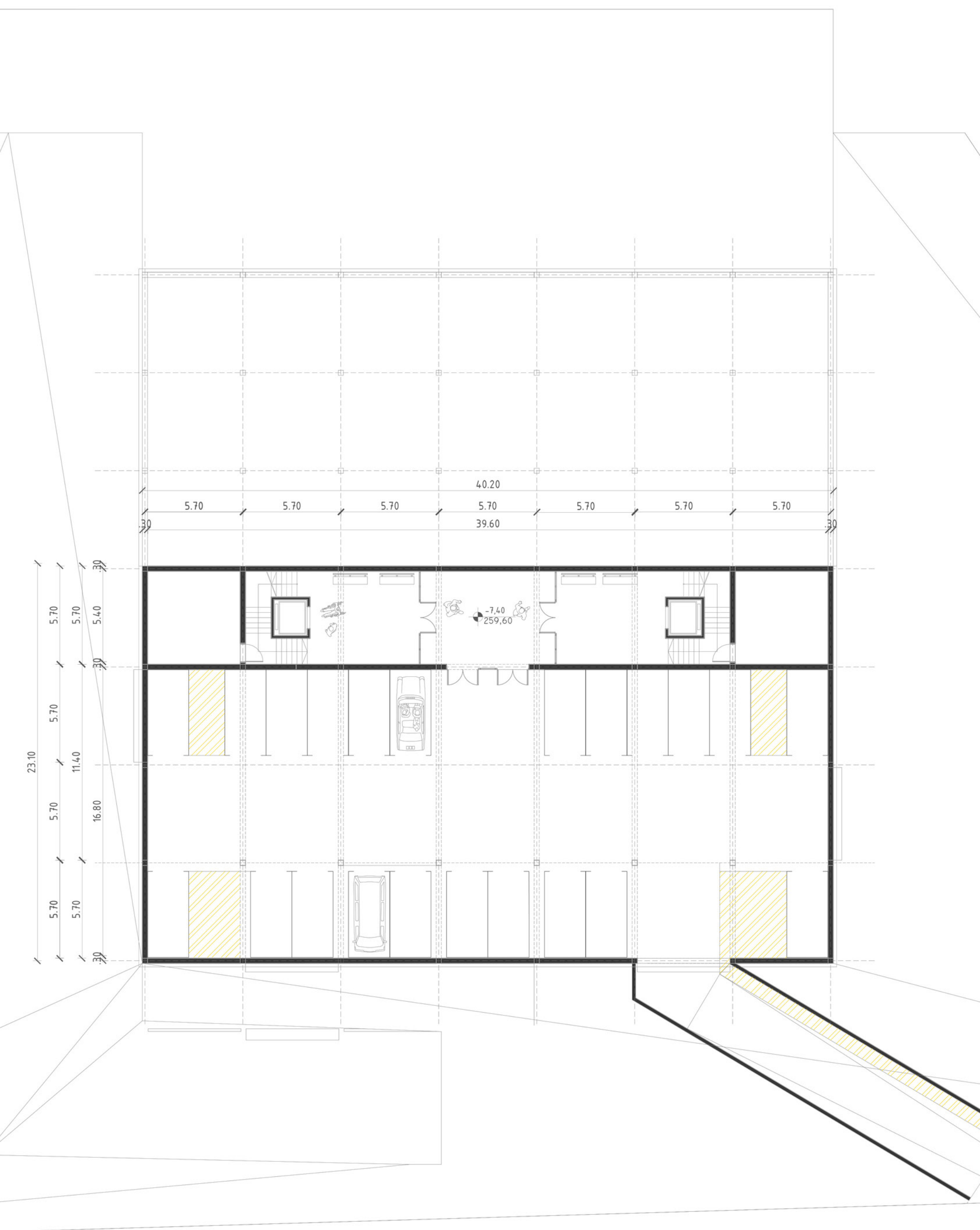
Basement -2 Garage Floor Plan 1:200
