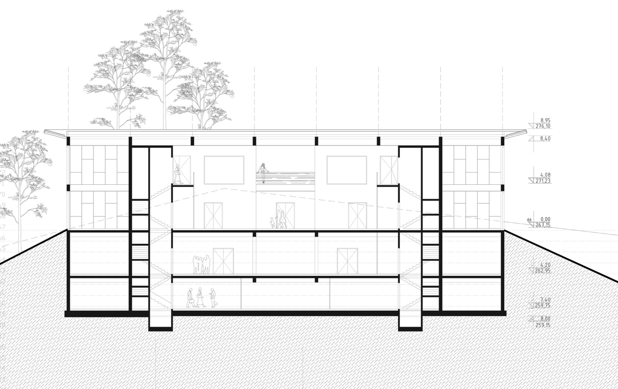
Section B-B 1:200
