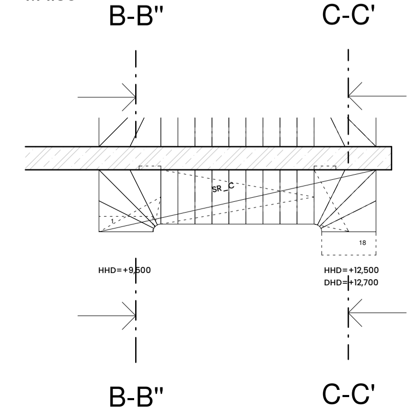
SCHODIŠTĚ_C M 1:50
